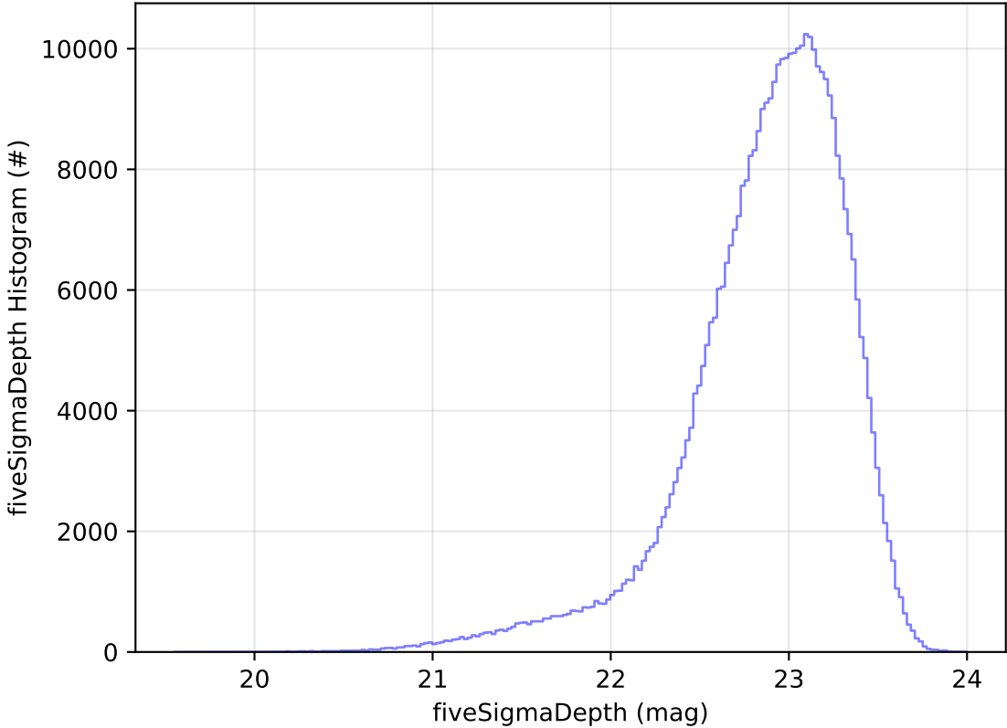
too_elab_r256_d3_griz_v3.4_10yrs All sky z band: fiveSigmaDepth Histogram
