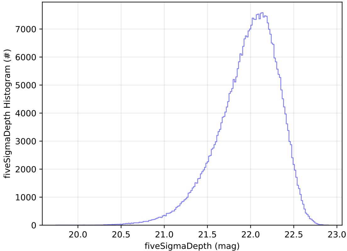
too_elab_r256_d3_griz_v3.4_10yrs All sky y band: fiveSigmaDepth Histogram
