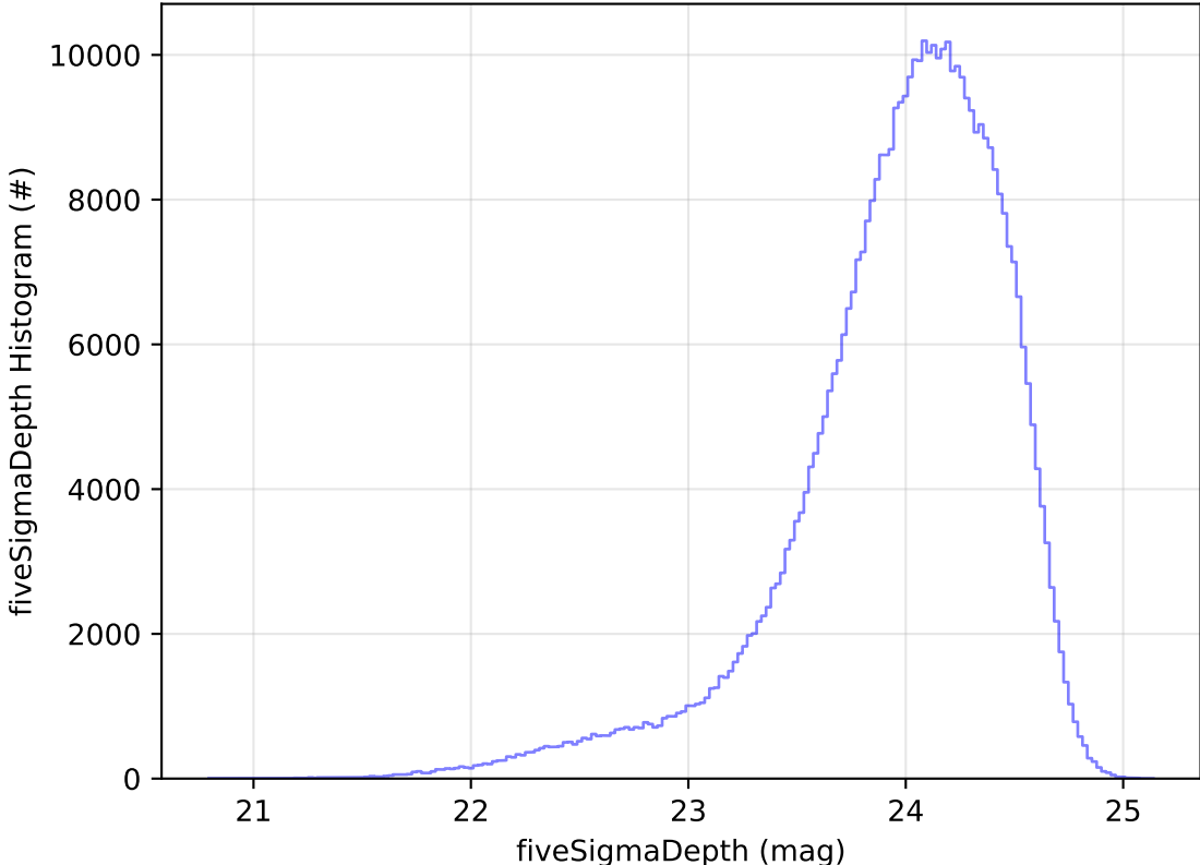
too_elab_r256_d3_griz_v3.4_10yrs All sky r band: fiveSigmaDepth Histogram
