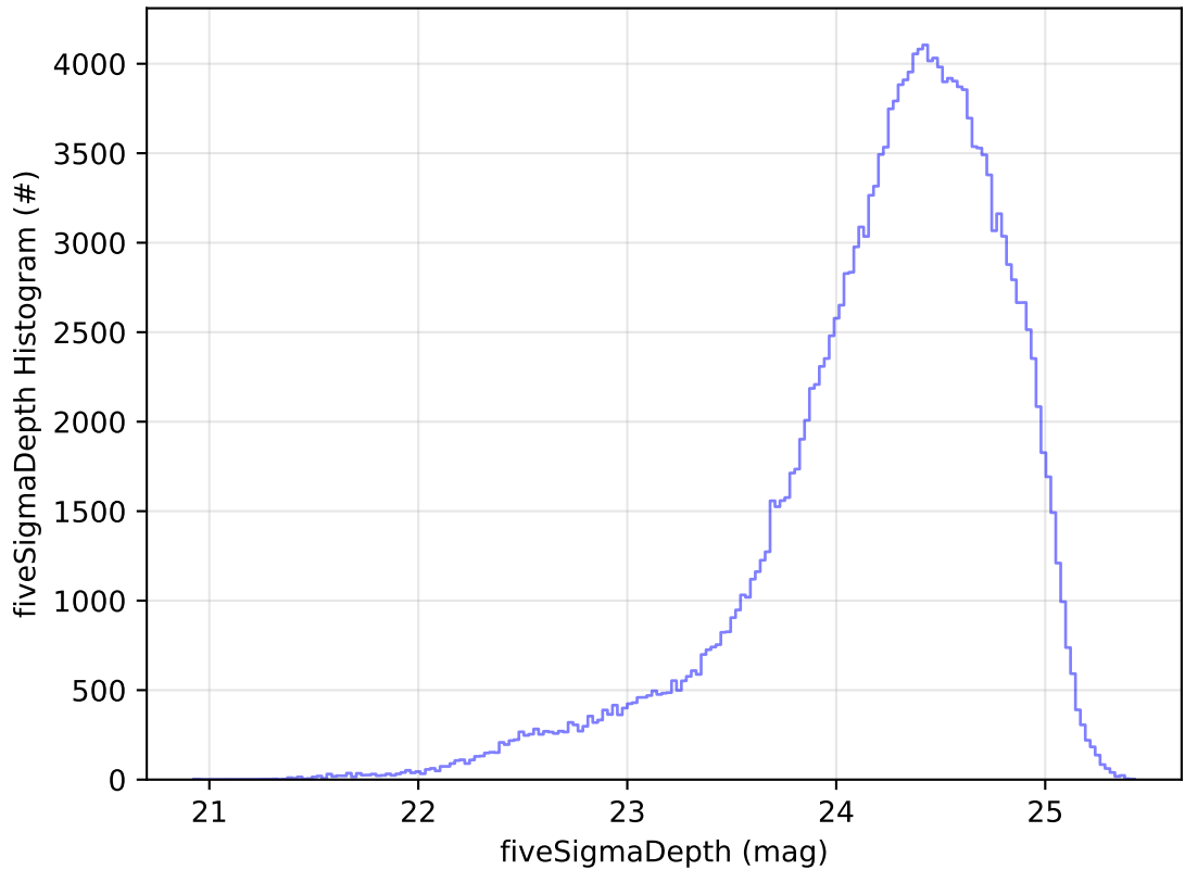
too_elab_r256_d3_griz_v3.4_10yrs All sky g band: fiveSigmaDepth Histogram
