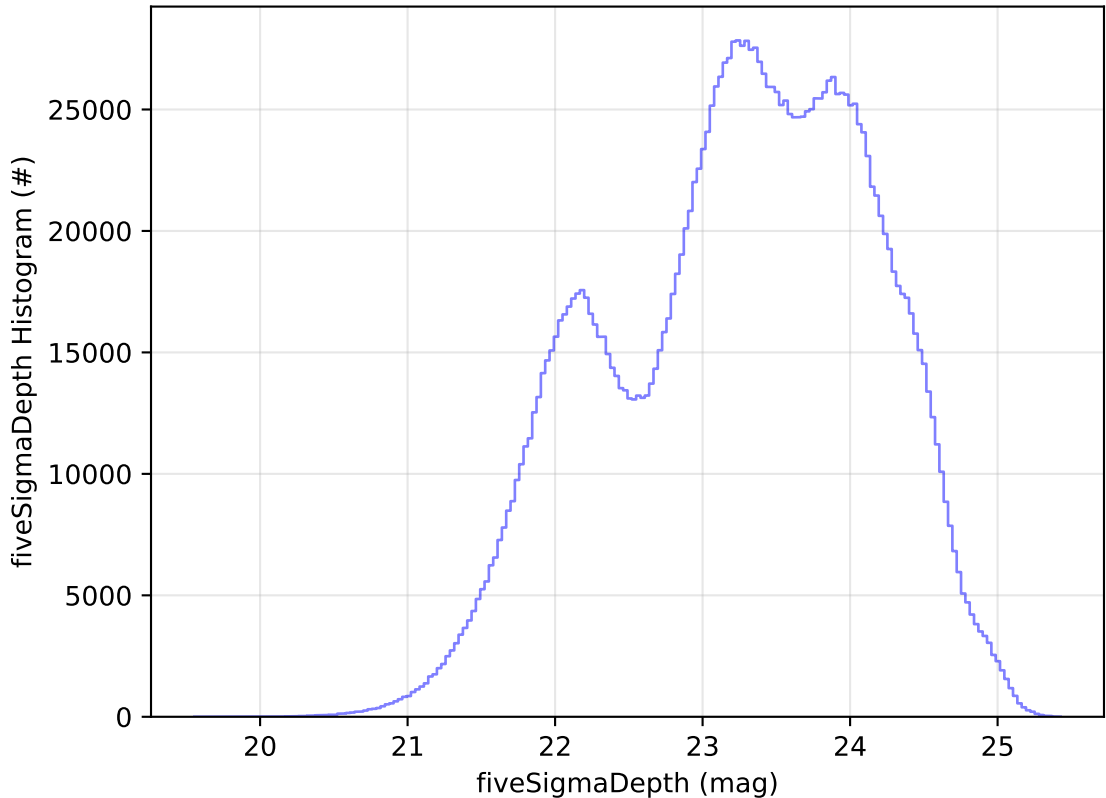
too_elab_r256_d3_griz_v3.4_10yrs All sky all bands: fiveSigmaDepth Histogram
