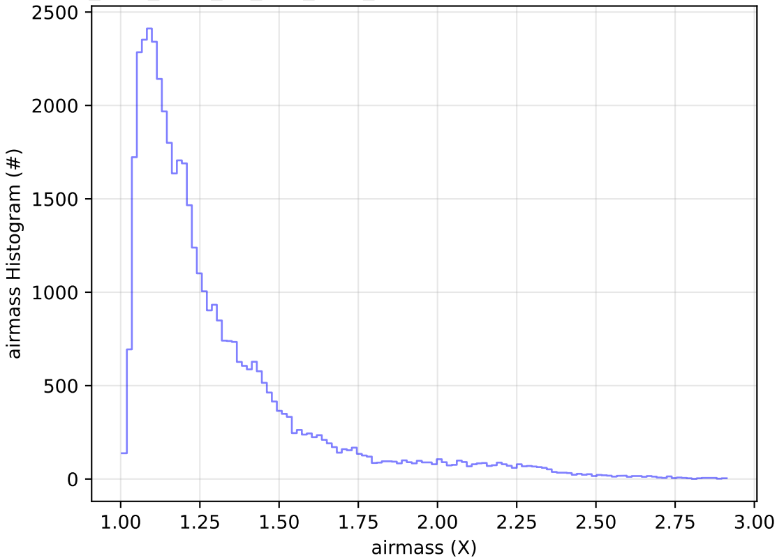
too_elab_r256_d3_griz_v3.4_10yrs Yr 1 z band: airmass Histogram
