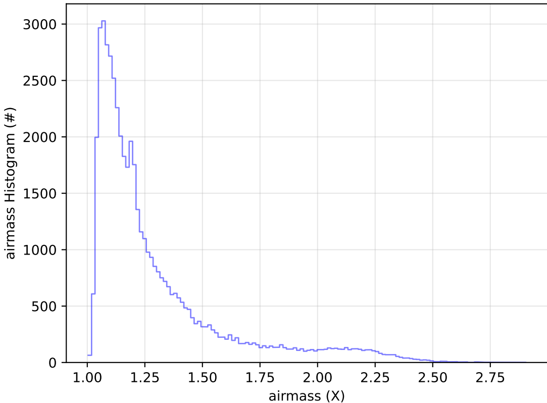
too_elab_r256_d3_griz_v3.4_10yrs Yr 1 r band: airmass Histogram
