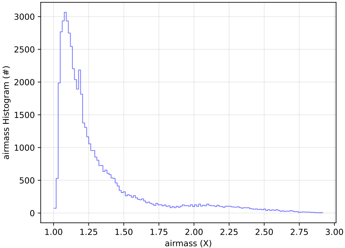
too_elab_r256_d3_griz_v3.4_10yrs Yr 1 i band: airmass Histogram
