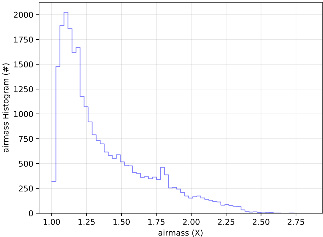
too_elab_r256_d3_griz_v3.4_10yrs Yr 1 g band: airmass Histogram
