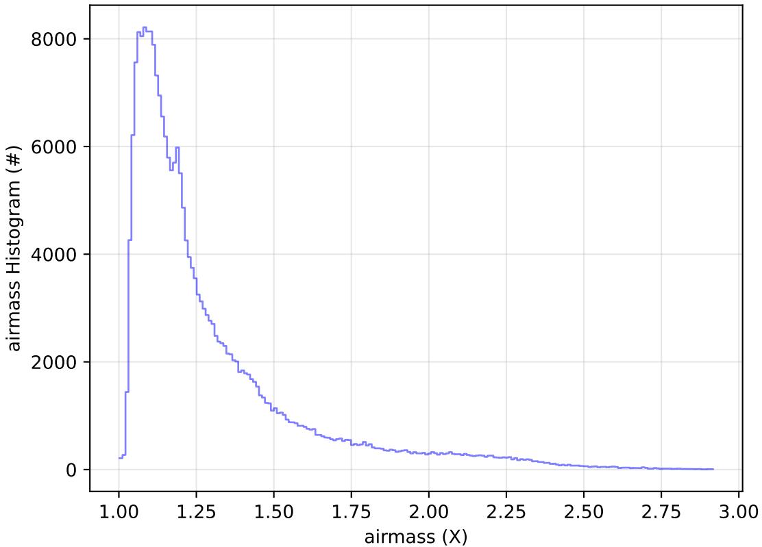
too_elab_r256_d3_griz_v3.4_10yrs Yr 1 all bands: airmass Histogram
