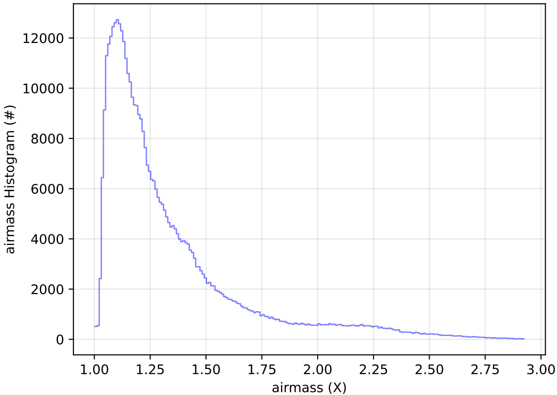
too_elab_r256_d3_griz_v3.4_10yrs WFD z band: airmass Histogram
