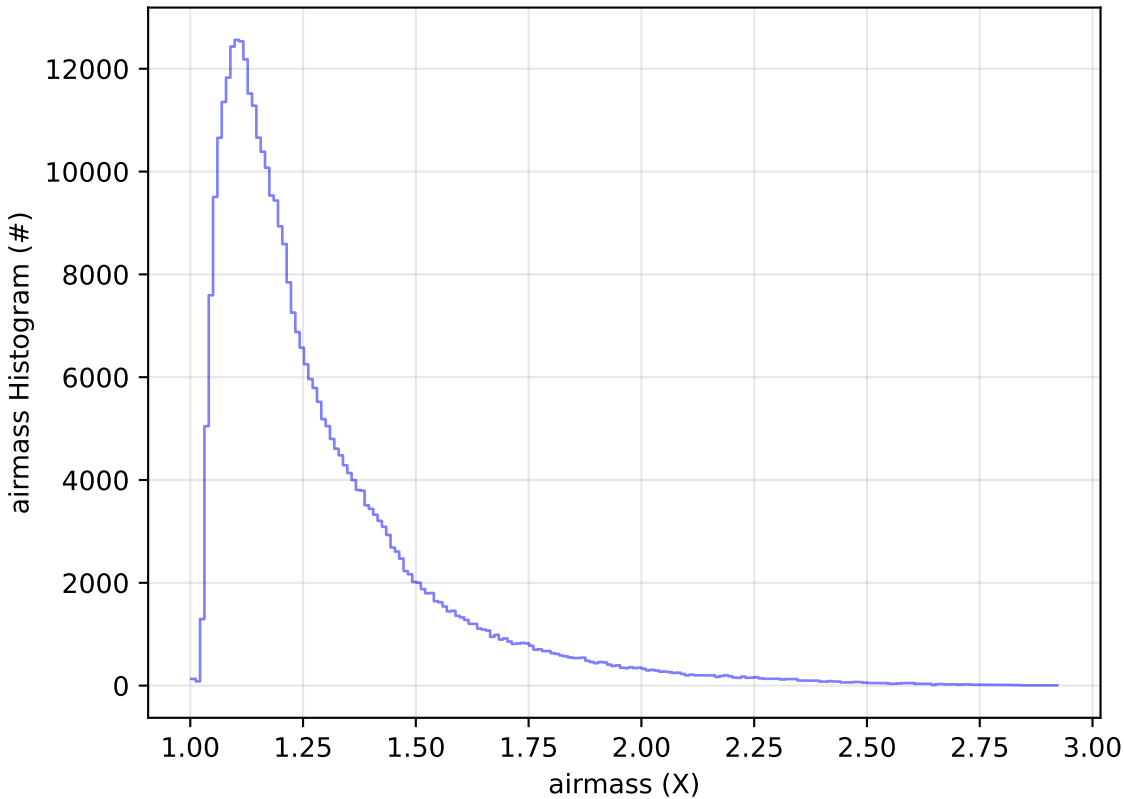
too_elab_r256_d3_griz_v3.4_10yrs WFD y band: airmass Histogram
