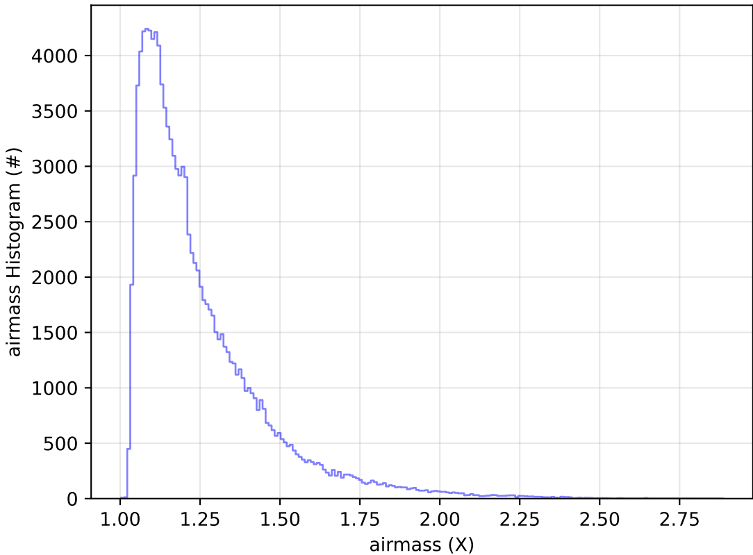
too_elab_r256_d3_griz_v3.4_10yrs WFD u band: airmass Histogram
