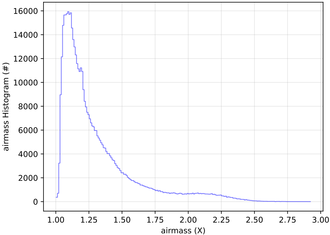
too_elab_r256_d3_griz_v3.4_10yrs WFD r band: airmass Histogram
