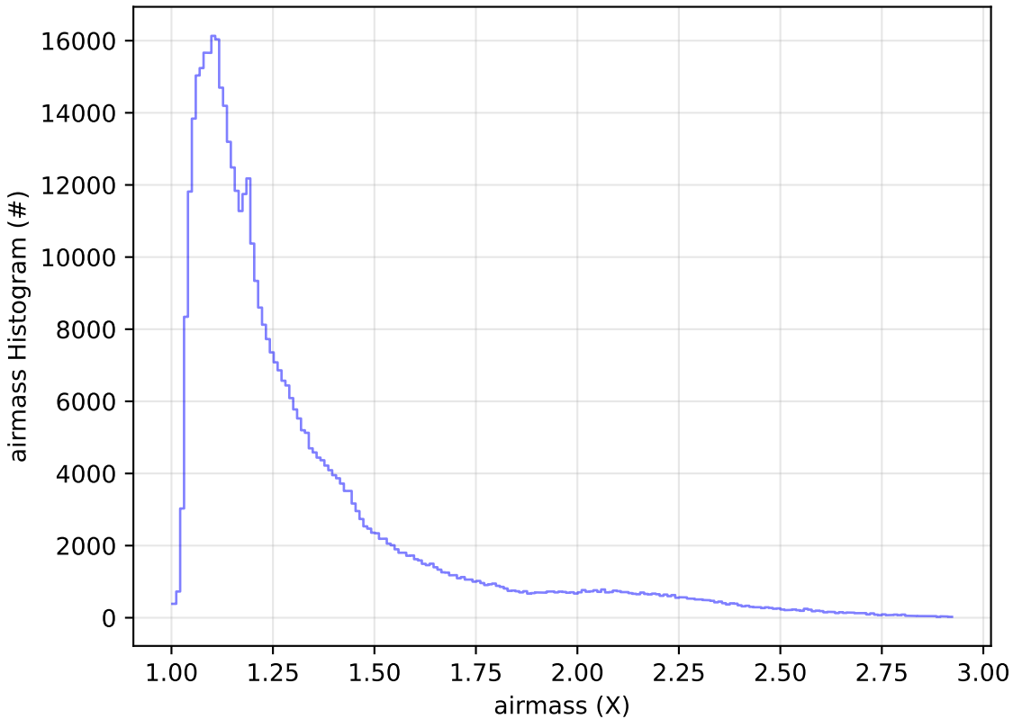
too_elab_r256_d3_griz_v3.4_10yrs WFD i band: airmass Histogram
