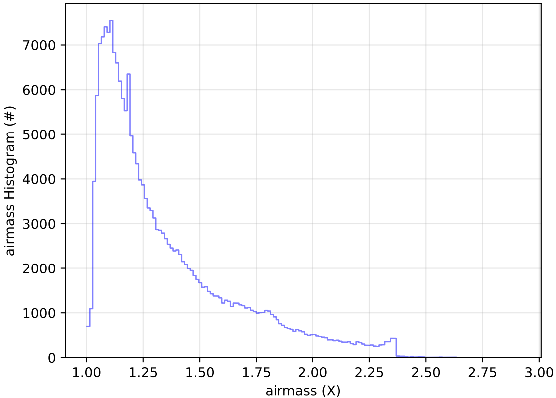
too_elab_r256_d3_griz_v3.4_10yrs WFD g band: airmass Histogram
