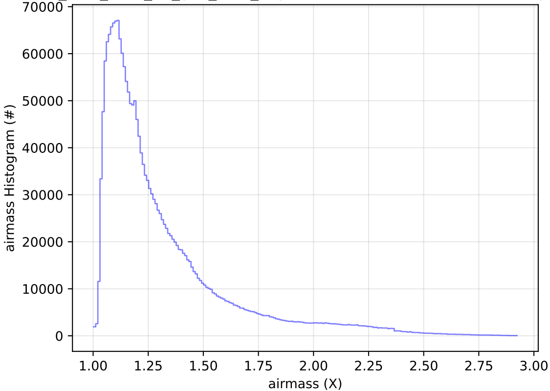
too_elab_r256_d3_griz_v3.4_10yrs WFD all bands: airmass Histogram
