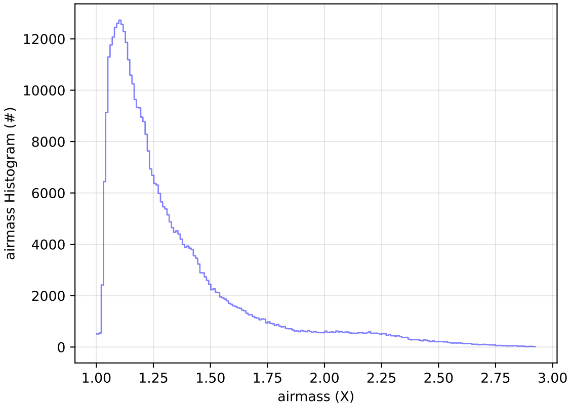
too_elab_r256_d3_griz_v3.4_10yrs All sky z band: airmass Histogram
