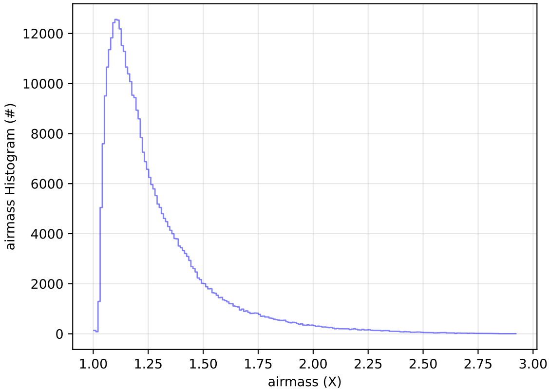
too_elab_r256_d3_griz_v3.4_10yrs All sky y band: airmass Histogram
