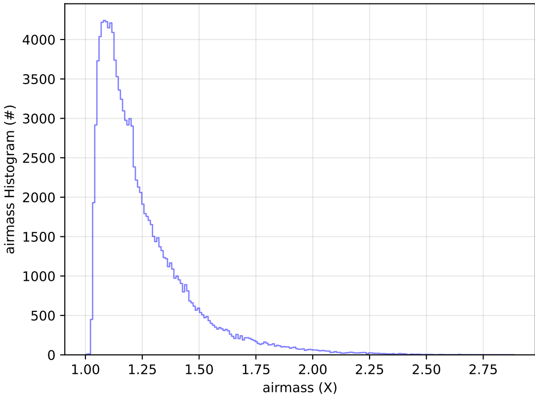
too_elab_r256_d3_griz_v3.4_10yrs All sky u band: airmass Histogram
