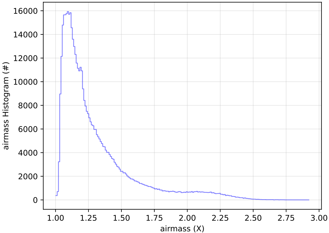
too_elab_r256_d3_griz_v3.4_10yrs All sky r band: airmass Histogram
