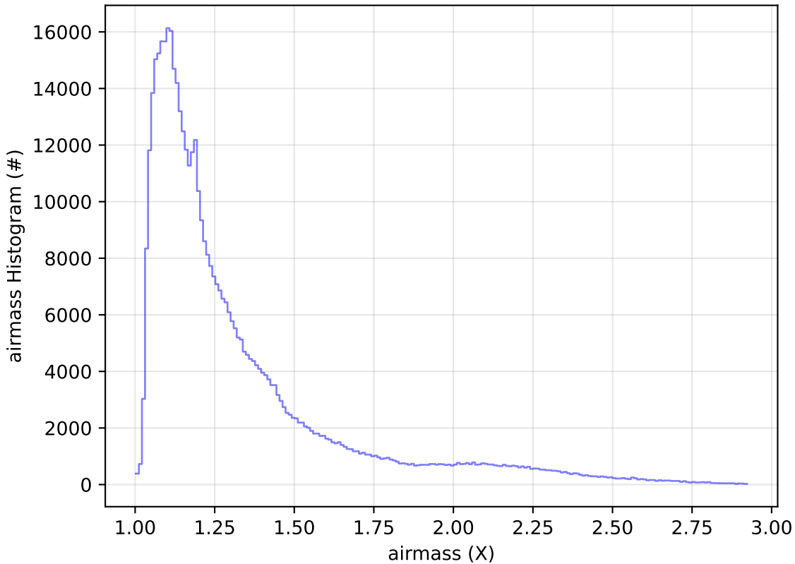
too_elab_r256_d3_griz_v3.4_10yrs All sky i band: airmass Histogram
