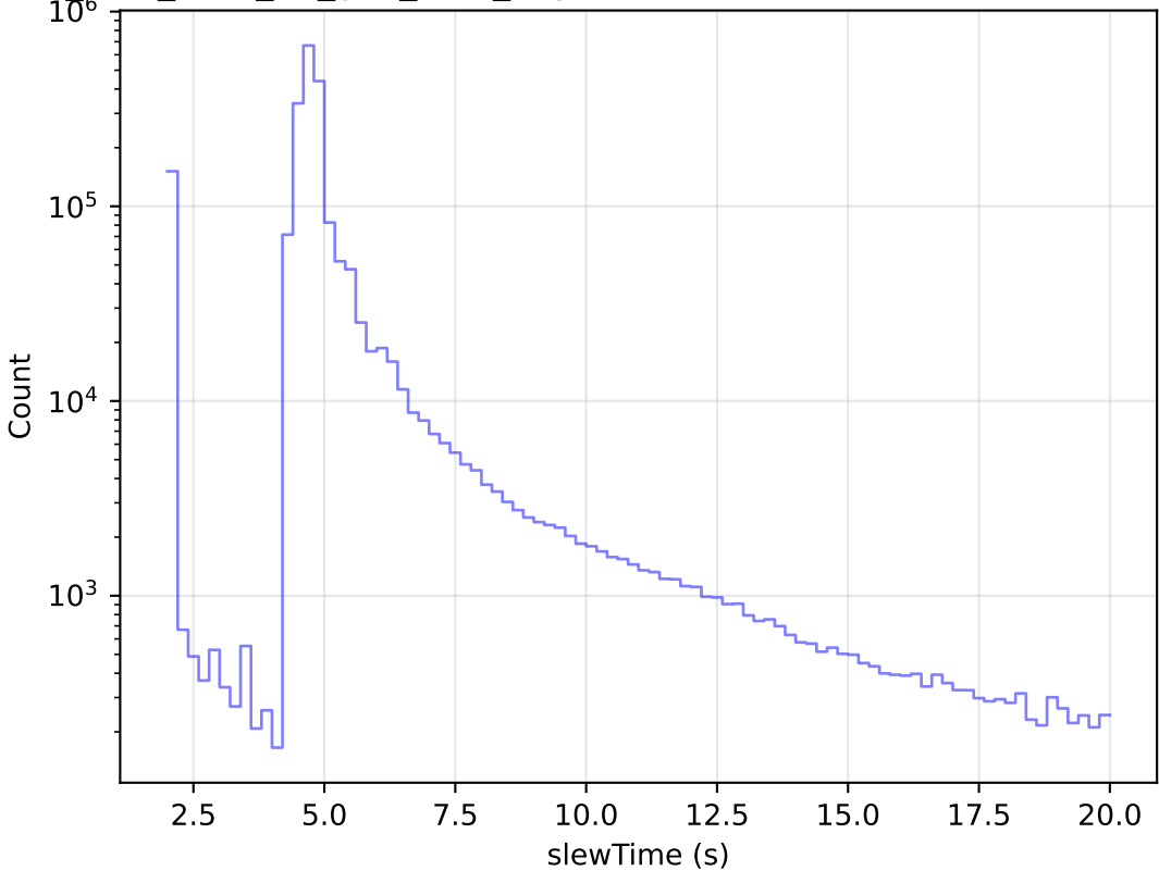
too_elab_r256_d3_griz_v3.4_10yrs All visits: Zoom Slew Time Histogram
