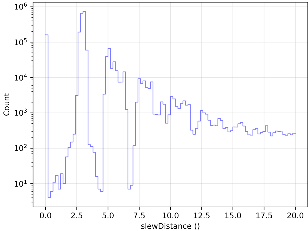
too_elab_r256_d3_griz_v3.4_10yrs All visits: Zoom Slew Distance Histogram
