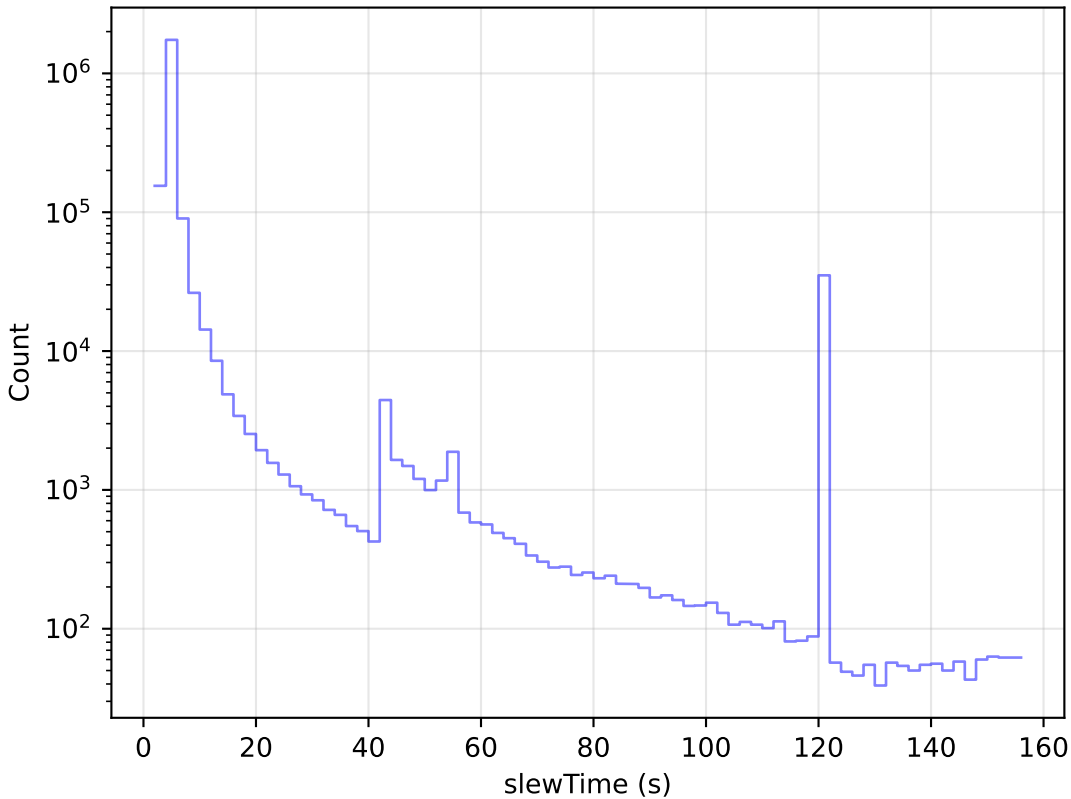
too_elab_r256_d3_griz_v3.4_10yrs All visits: Slew Time Histogram
