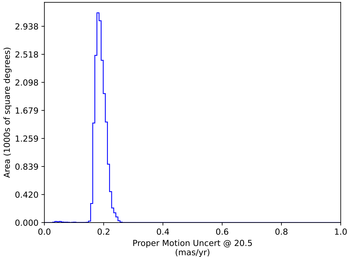
too_elab_r256_d3_griz_v3.4_10yrs WFD: Proper Motion Uncert @ 20.5
