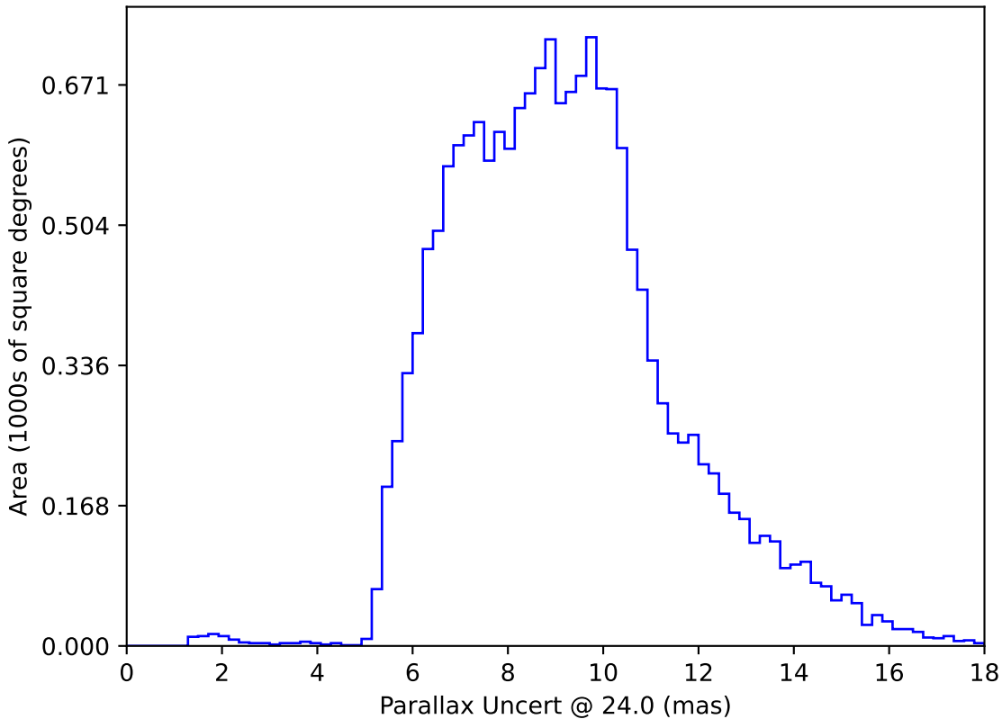
too_elab_r256_d3_griz_v3.4_10yrs WFD: Parallax Uncert @ 24.0
