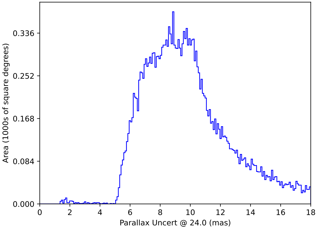
too_elab_r256_d3_griz_v3.4_10yrs All sky: Parallax Uncert @ 24.0
