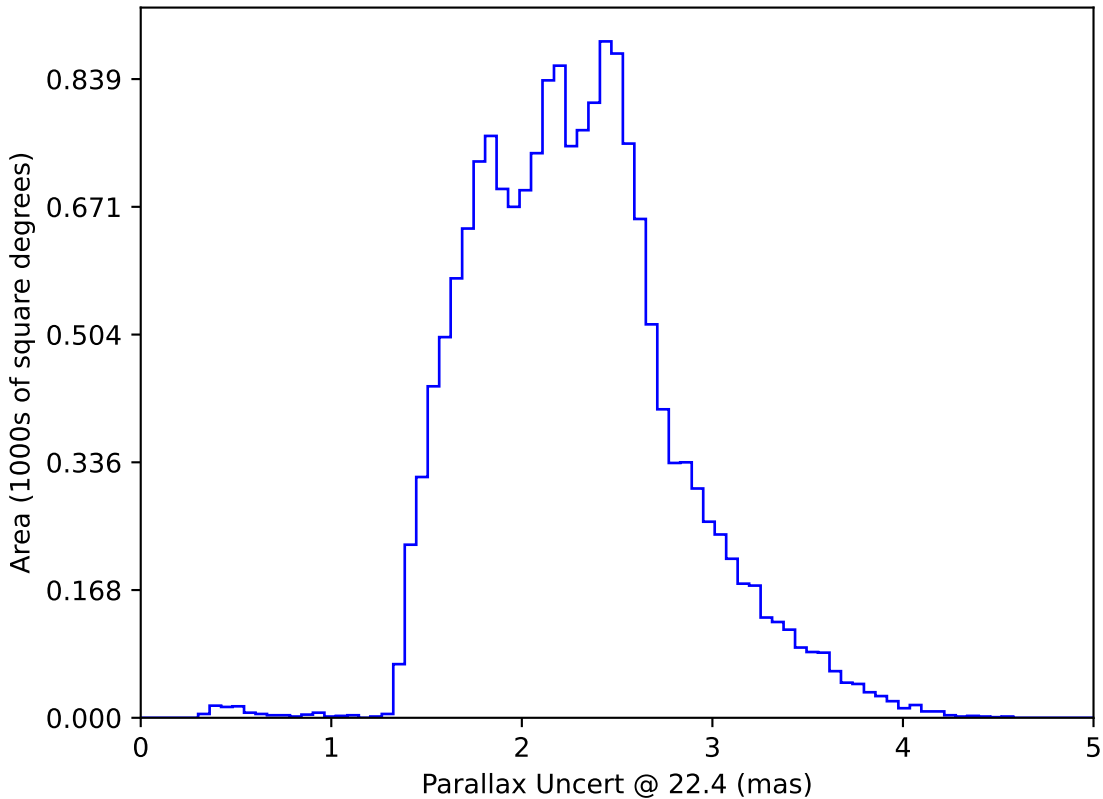
too_elab_r256_d3_griz_v3.4_10yrs WFD: Parallax Uncert @ 22.4
