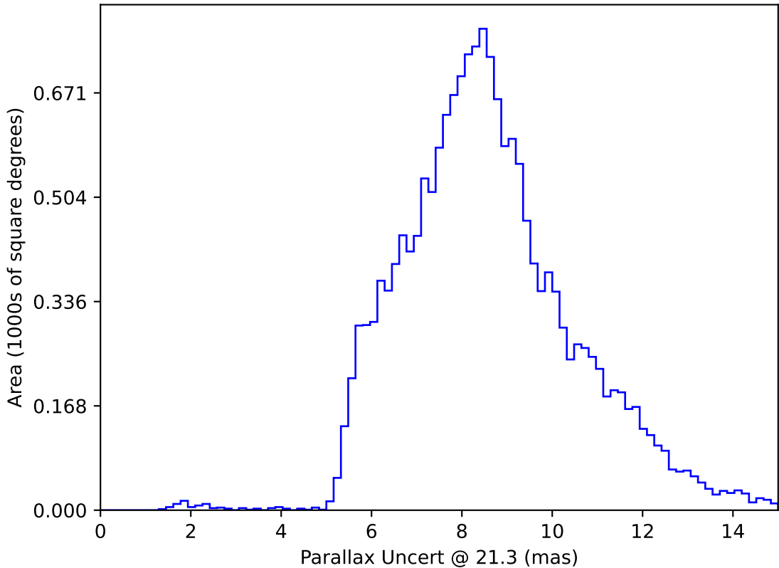
too_elab_r256_d3_griz_v3.4_10yrs WFD y band only: Parallax Uncert @ 21.3
