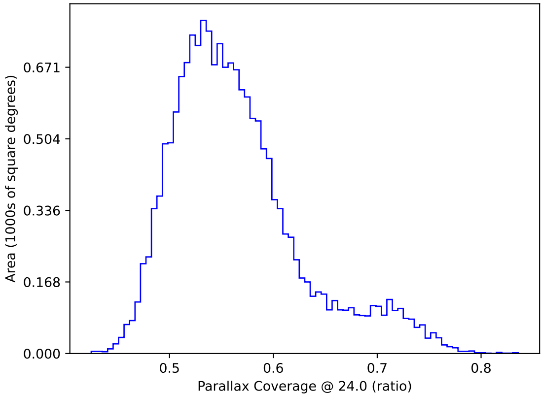
too_elab_r256_d3_griz_v3.4_10yrs WFD: Parallax Coverage @ 24.0
