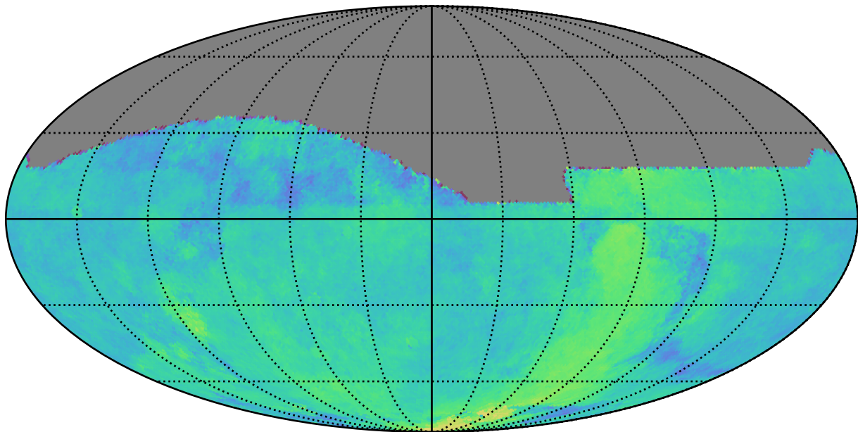
too_elab_r256_d3_griz_v3.4_10yrs All sky: Parallax Coverage @ 24.0
