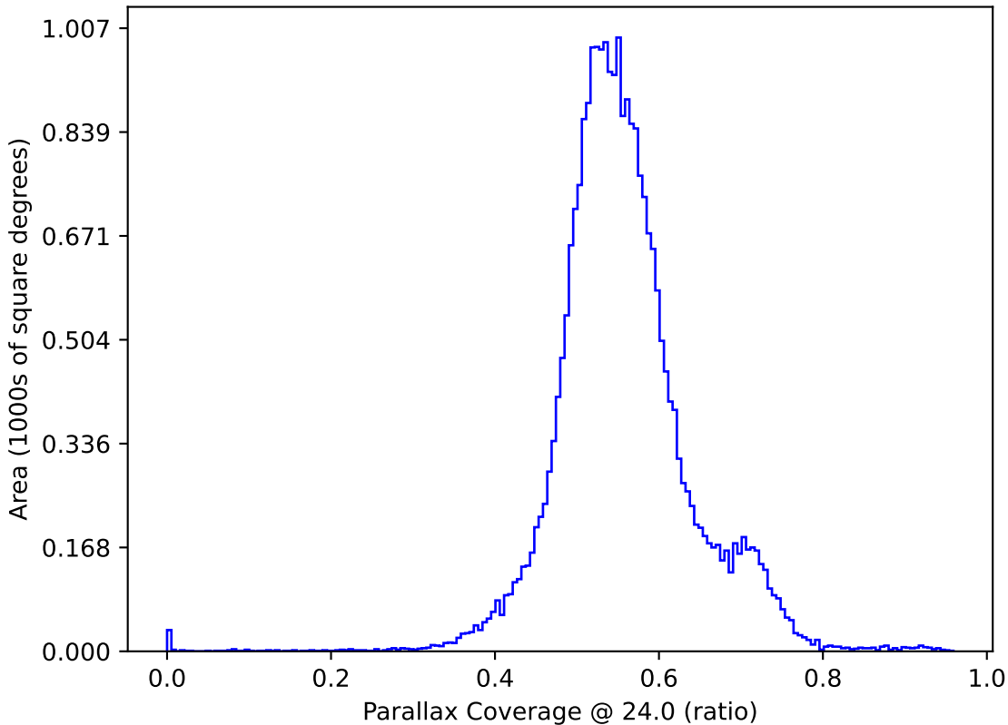
too_elab_r256_d3_griz_v3.4_10yrs All sky: Parallax Coverage @ 24.0
