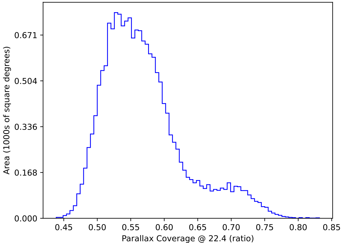
too_elab_r256_d3_griz_v3.4_10yrs WFD: Parallax Coverage @ 22.4
