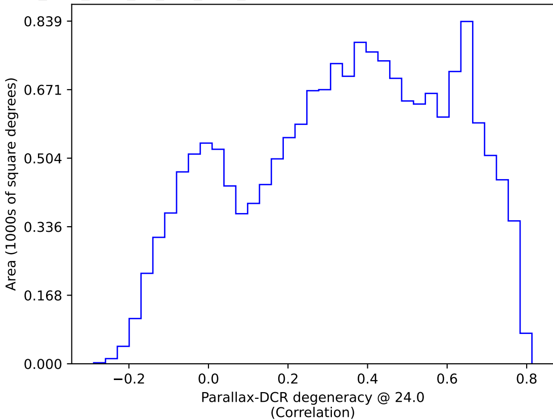
too_elab_r256_d3_griz_v3.4_10yrs WFD: Parallax-DCR degeneracy @ 24.0
