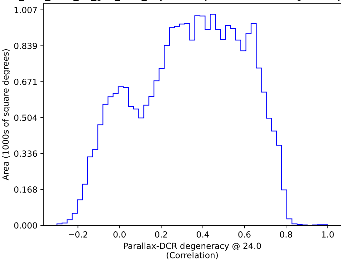
too_elab_r256_d3_griz_v3.4_10yrs All sky: Parallax-DCR degeneracy @ 24.0
