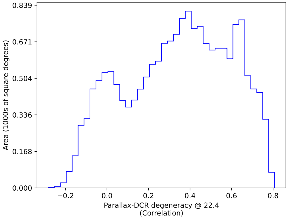
too_elab_r256_d3_griz_v3.4_10yrs WFD: Parallax-DCR degeneracy @ 22.4
