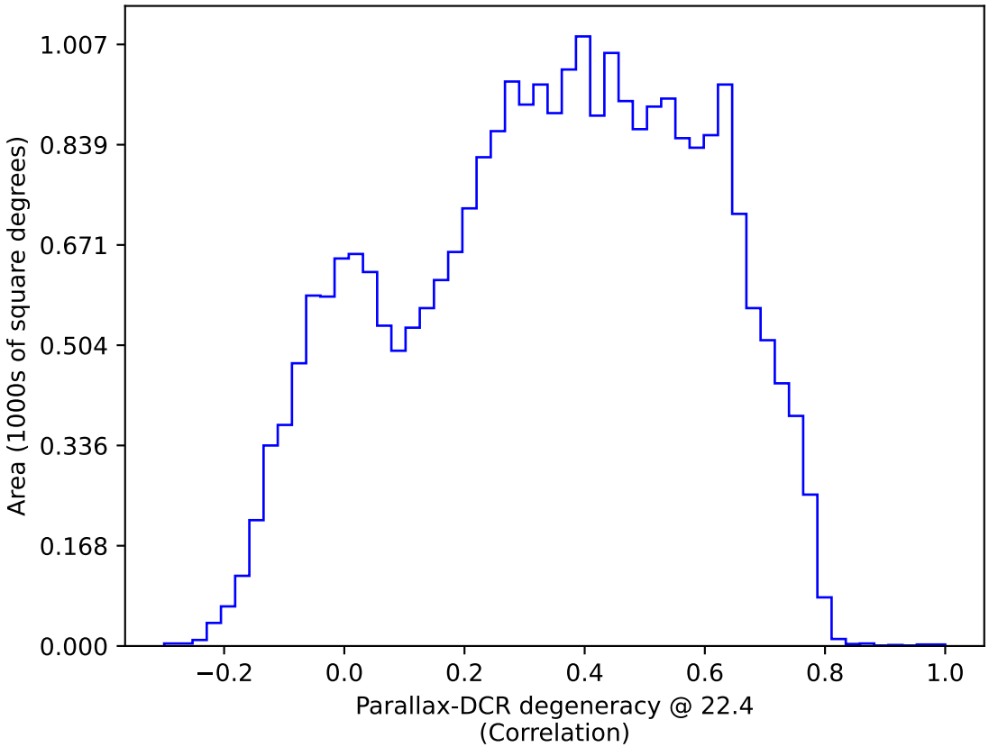
too_elab_r256_d3_griz_v3.4_10yrs All sky: Parallax-DCR degeneracy @ 22.4
