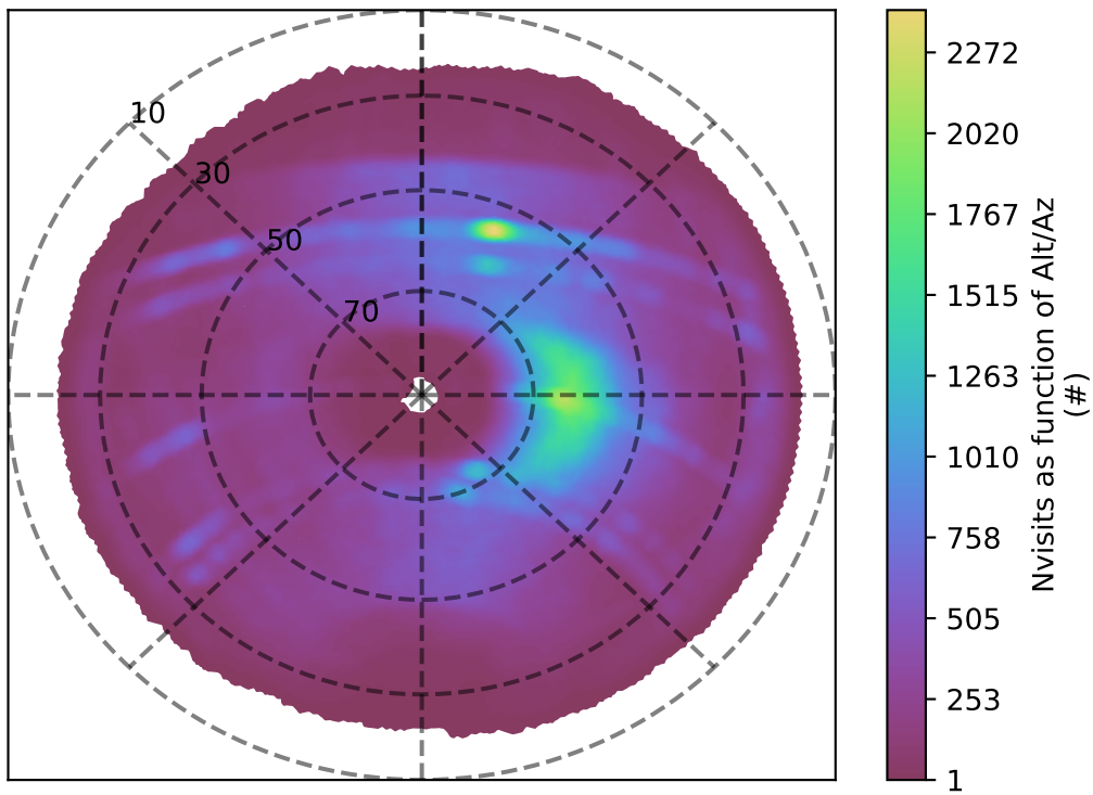
too_elab_r256_d3_griz_v3.4_10yrs z band: Nvisits as function of Alt/Az
