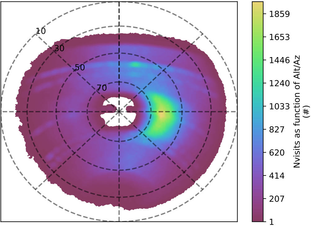
too_elab_r256_d3_griz_v3.4_10yrs y band: Nvisits as function of Alt/Az
