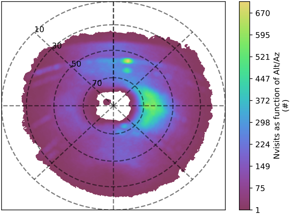
too_elab_r256_d3_griz_v3.4_10yrs u band: Nvisits as function of Alt/Az
