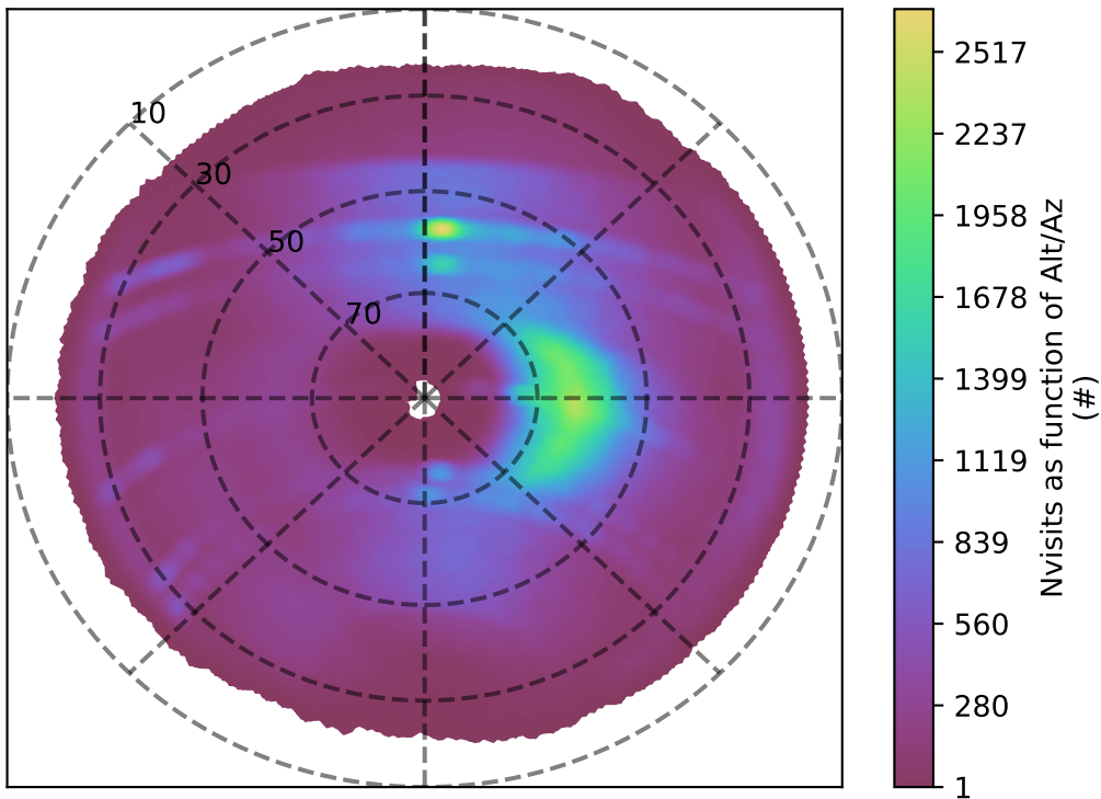
too_elab_r256_d3_griz_v3.4_10yrs i band: Nvisits as function of Alt/Az
