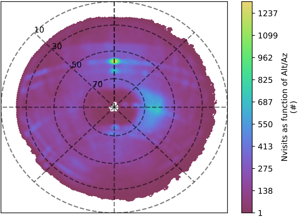
too_elab_r256_d3_griz_v3.4_10yrs g band: Nvisits as function of Alt/Az
