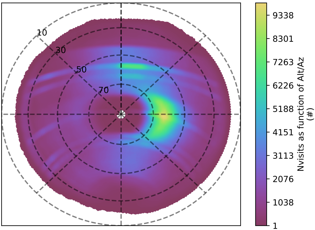
too_elab_r256_d3_griz_v3.4_10yrs all bands: Nvisits as function of Alt/Az
