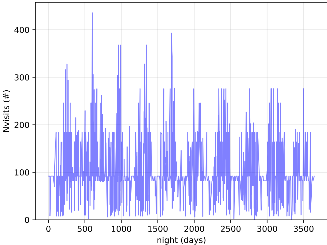
too_elab_r256_d3_griz_v3.4_10yrs DDF: Nvisits
