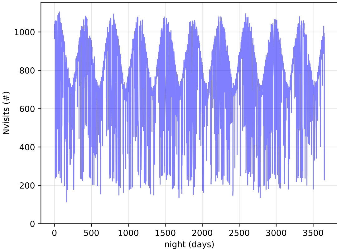
too_elab_r256_d3_griz_v3.4_10yrs All visits: Nvisits
