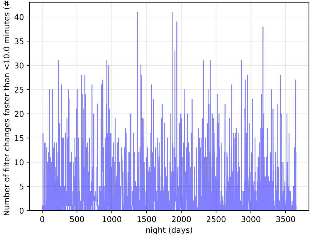
too_elab_r256_d3_griz_v3.4_10yrs Per Night: Number of filter changes faster than <10.0 minutes
