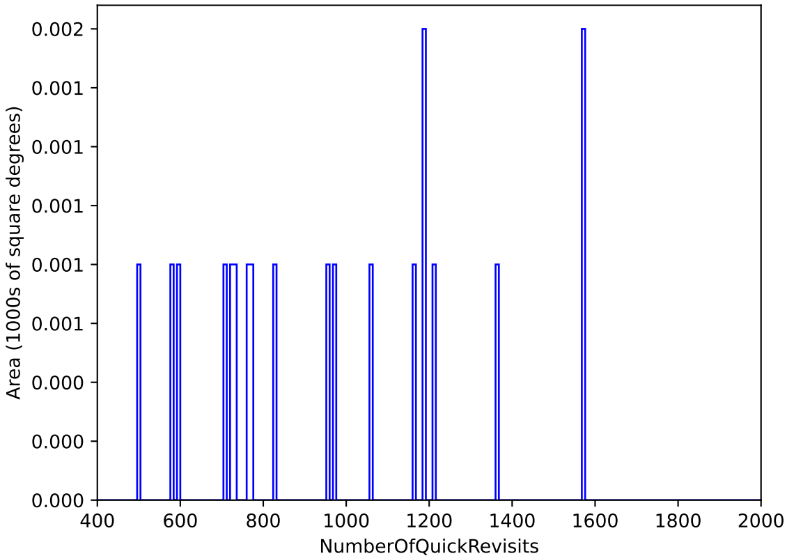
too_elab_r256_d3_griz_v3.4_10yrs WFD: NumberOfQuickRevisits
