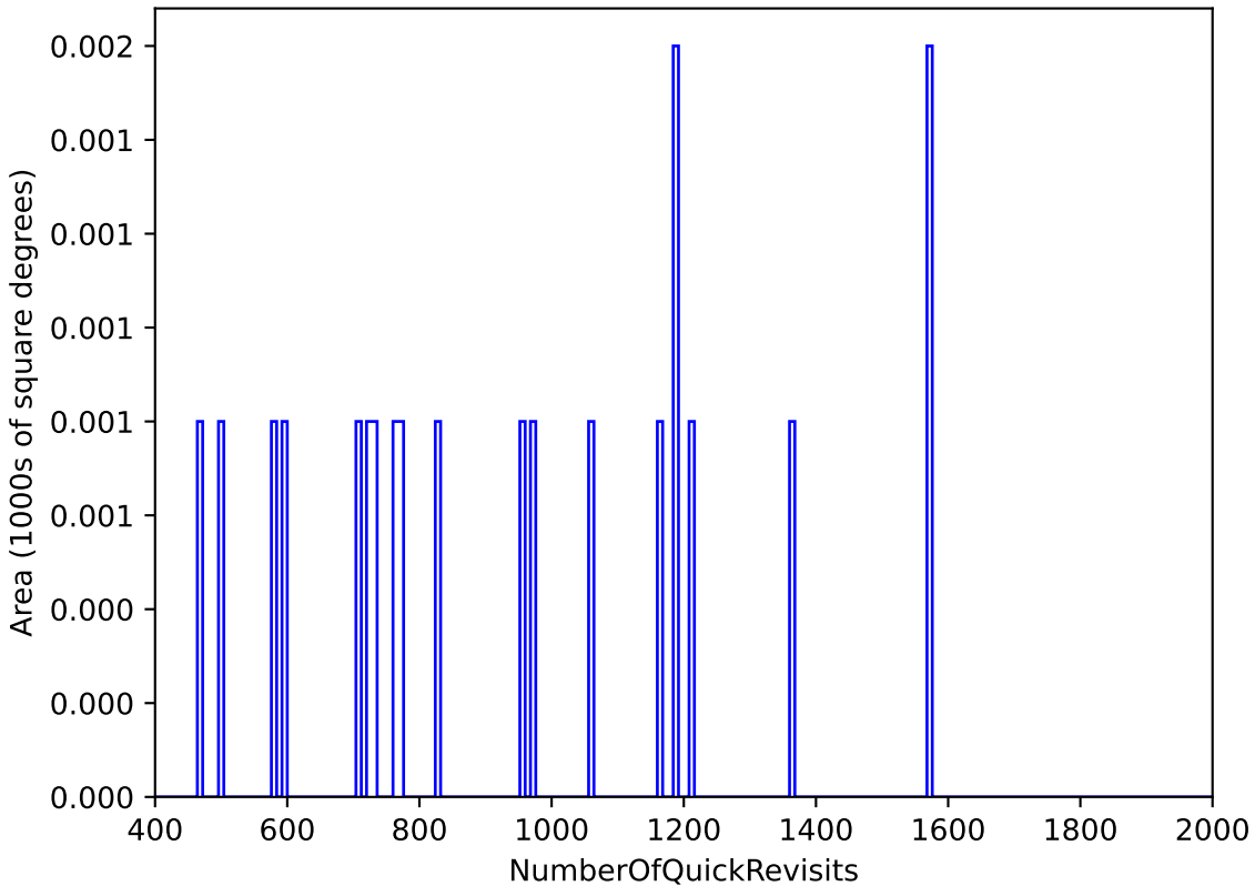
too_elab_r256_d3_griz_v3.4_10yrs All sky: NumberOfQuickRevisits
