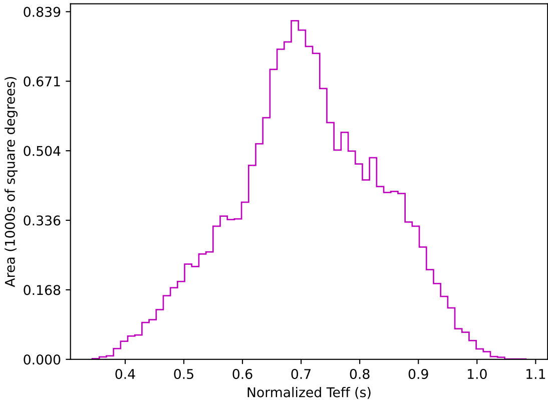
too_elab_r256_d3_griz_v3.4_10yrs WFD z band: Normalized Teff
